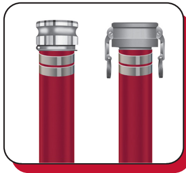
Red PVC Layflat Water Discharge Aluminum Male X Female Cam
