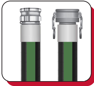
Rubber Water Suction Aluminum Male X Female Cam
